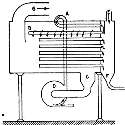
FIG. 20.—Vacuum concentration of liquors.
